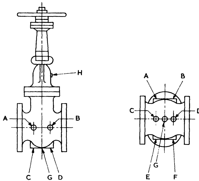
Figure 3 — Location of tappings
